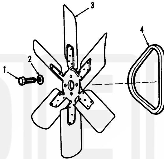
Figure 53A. Engine cooling fan and belt.
